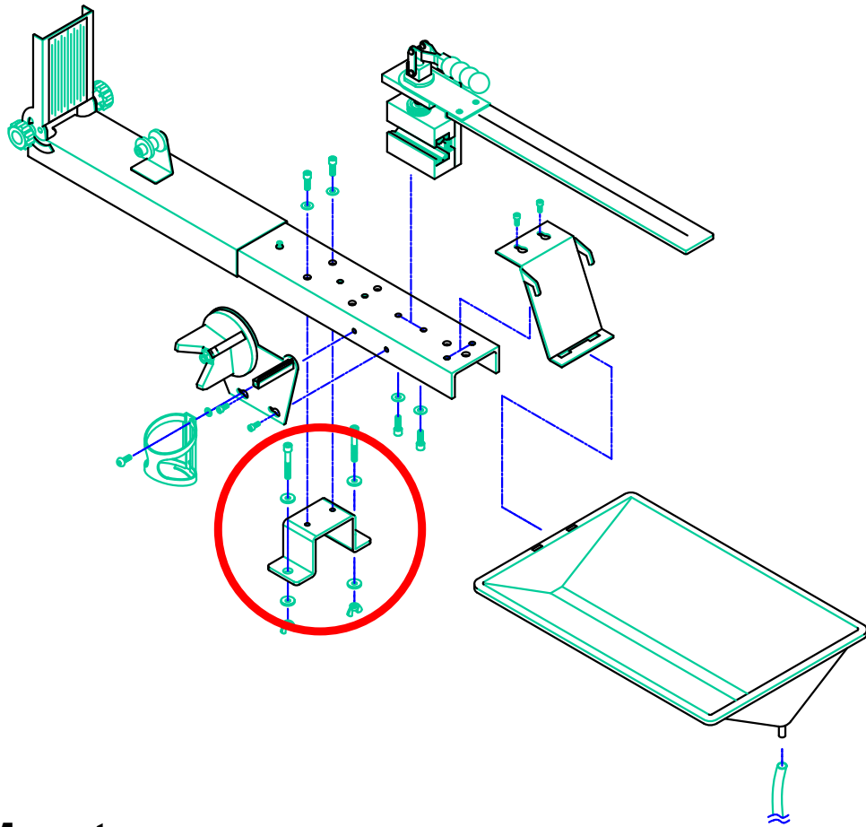
Bench Mount
